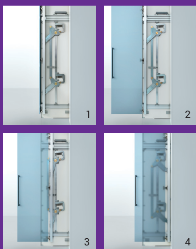
Mechanism movement as door exits recess
